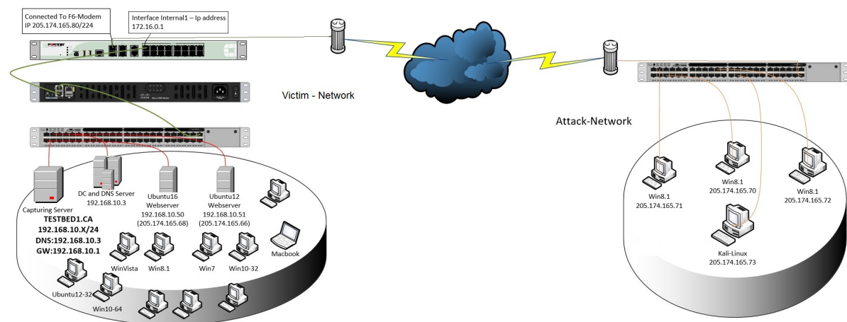
Figure 1: Testbed Architecture.
